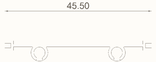
Polycarbonate Led profile (36 WATT)
